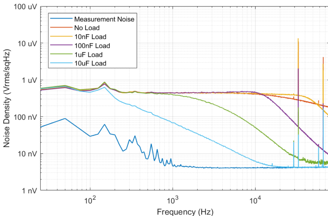
Figure 8. Output noise density for a range of load conditions in \text{V}_{\text{rms}}/\sqrt{\text{Hz}}
