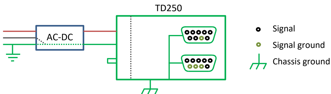
Figure 3. TD250 Chassis and signal ground configuration
