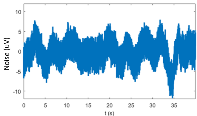
Figure 6. Total noise with a 350 Ohm Bridge (0.1Hz to 100Hz)
