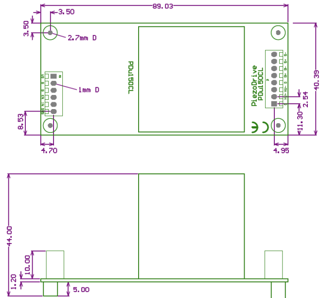
Figure 11. Dimensions (mm)
