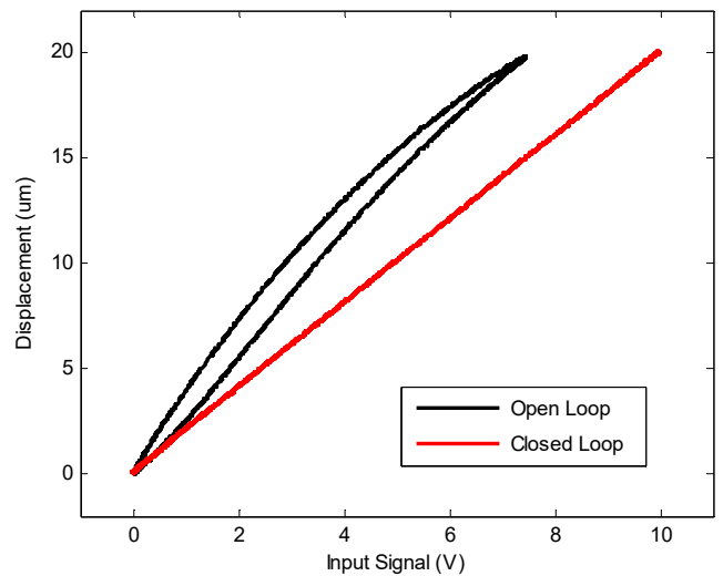
Figure 9. Open- and Closed-Loop response (1-Hz Sinusoid)
