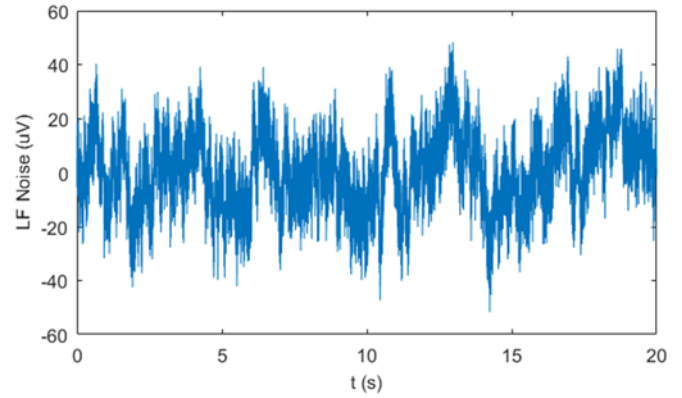
Figure 5. Low frequency output noise (0.03 Hz to 10 Hz)
