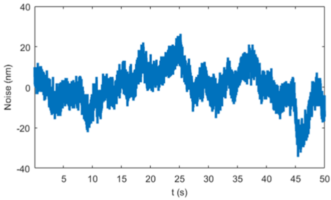
Figure 10. Closed-loop positioning noise (0.03Hz to 1MHz)
