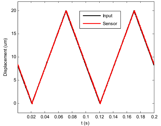
Figure 8. 10-Hz Full-Range Tracking Performance
