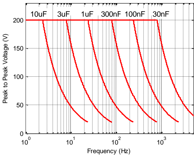
Figure 4. Power bandwidth
