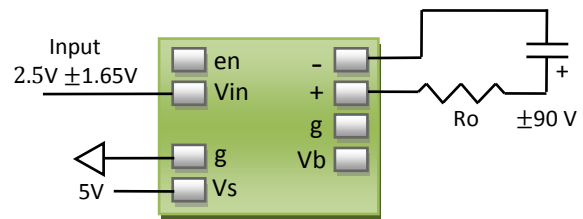
\pm 90 V Piezo bender driver
