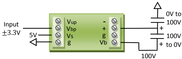
100 V Three-wire bender driver with bias
