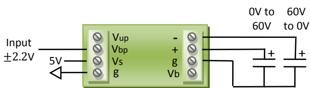
60 V Push-pull stack driver or bender driver
