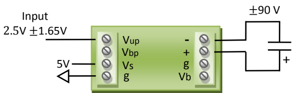
±90 V Piezo bender driver with unipolar input
